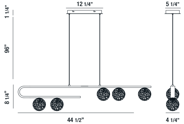
37351-014 5-LIGHT LINEAR LED CHANDELIER 15W/LED 3500K/1200lm (dimmable)
