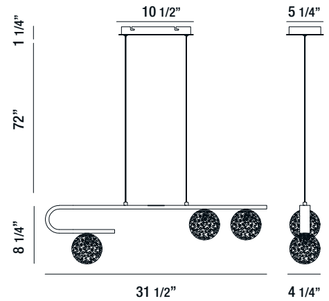
37350-017 3-LIGHT LINEAR LED CHANDELIER 9W/LED 3500K/720lm (dimmable)
