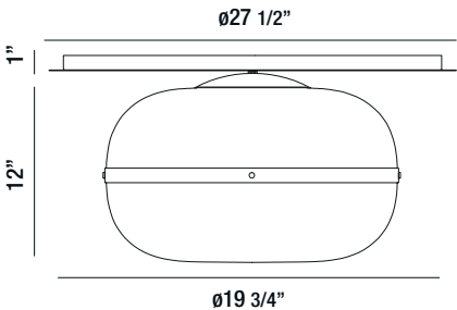
37088-019 3-LIGHT LARGE FLUSHMOUNT 3 x 60W/EDISON BULB E26/120V (included)
