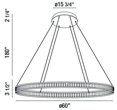
37093-013 LARGE LED CHANDELIER 135W/LED 3000K/8100lm (dimmable)
