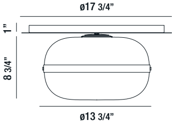
37087-012 1-LIGHT MEDIUM FLUSHMOUNT 1 x 60W/EDISON BULB E26/120V (included)
