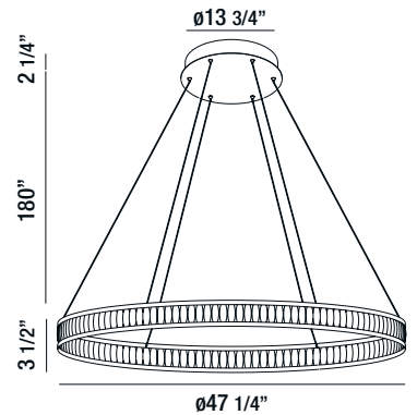
37092-016 MEDIUM LED CHANDELIER 105W/LED 3000K/6300lm (dimmable)
