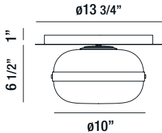
37086-015 1-LIGHT SMALL FLUSHMOUNT 1 x 60W/EDISON BULB E26/120V (included)
