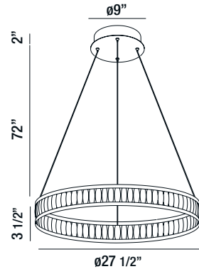
37091-019 SMALL LED CHANDELIER 60W/LED 3000K/3600lm (dimmable)
