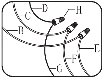
Wire connection
